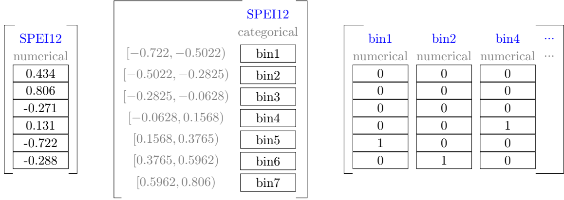
Figure A.3: Example of discretization of 12 months timescale of SPEI
