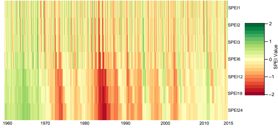
Figure 5: SPEI timescales for 55 years in six western African countries.
