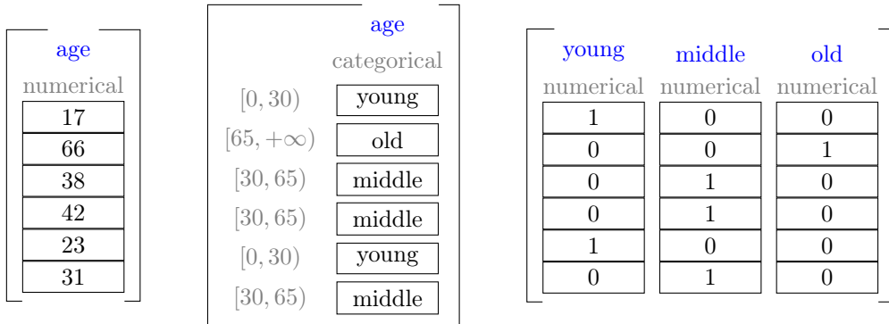
Figure A.2: Example of one-hot encoding and binarization of the variable age
