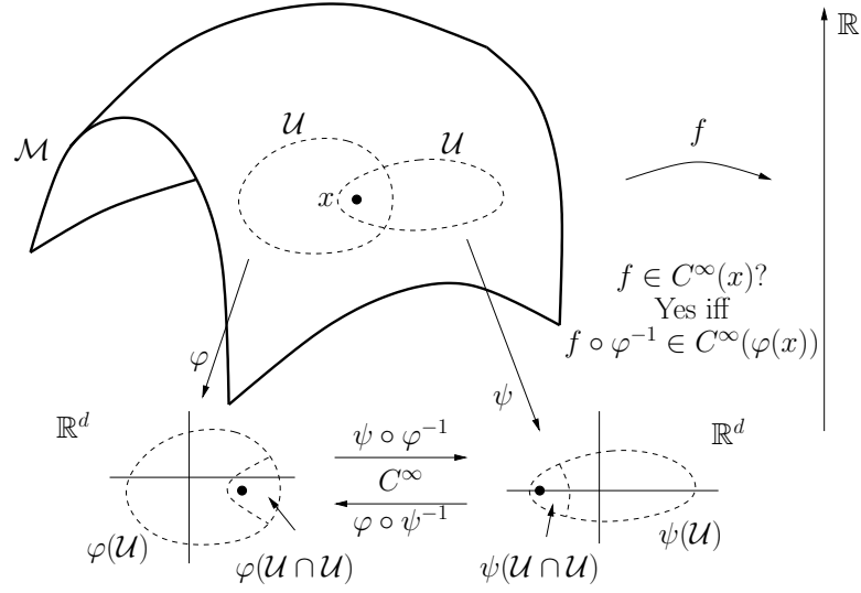
Fig. 4. Manifold structures and smoothness of objective functions.
