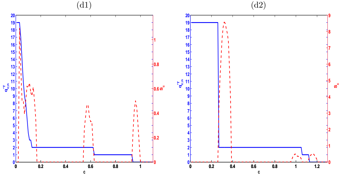
Figure 3: Example 2. AR loadings, q = 2 , n = 150 , T = 120 ; M_T = [0.5\sqrt{T}] . Simultaneous plots of c \mapsto S_c and c \mapsto q_{c,n}^{*T} for penalty function p_3(n, T) := \left( \min [n, M_T^2, M_T^{-1/2}T^{1/2}] \right)^{-1} \log \left( \min [n, M_T^2, M_T^{-1/2}T^{1/2}] \right) , q_{\max} = 19 , and (d1) IC_{1;n}^{*T}(k) criterion, (d2) IC_{2;n}^{*T}(k) criterion, respectively.
