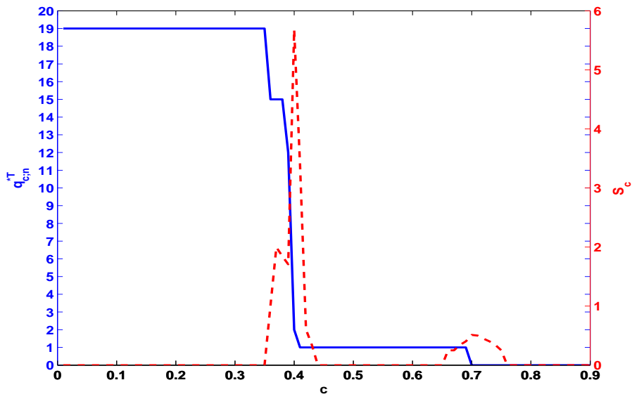
Figure 4: Eurozone macroeconomic indicators ( n = 62 , T = 40 ). Simultaneous plots of c \mapsto S_c and c \mapsto q_{c,n}^{*T} for n_j = 47 + j , j = 1, \dots, 12 , M_T = [0.5\sqrt{T}] = 3 , penalty function p_1(n, T) = (M_T^{-2} + M_T^{1/2}T^{-1/2} + n^{-1}) \log(\min[n, M_T^2, M_T^{-1/2}T^{1/2}]) , and the IC_{2;n}^{*T}(k) criterion, respectively.
