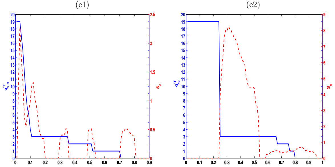
Figure 2: Example 1. MA loadings, q = 3 , n = T = 200 ; M_T = [0.7\sqrt{T}] . Simultaneous plots of c \mapsto S_c and c \mapsto q_{c,n}^{*T} , using penalty function p_3(n, T) := \left( \min [n, M_T^2, M_T^{-1/2}T^{1/2}] \right)^{-1} \log \left( \min [n, M_T^2, M_T^{-1/2}T^{1/2}] \right) , q_{\max} = 19 , and (c1) IC_{1;n}^{*T}(k) criterion, (c2) IC_{2;n}^{*T}(k) criterion, respectively.
