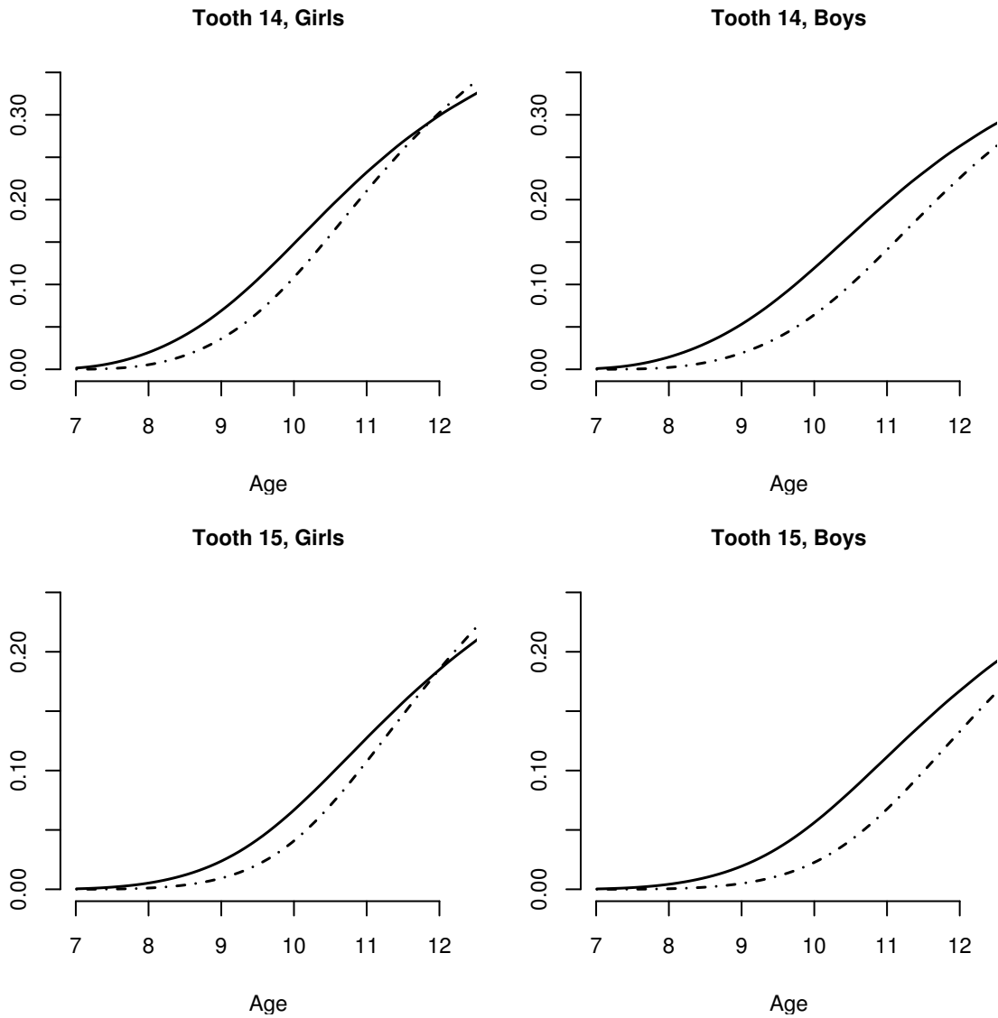
FIGURE 3. Predictive hazard curves of emergence based on the model gender * dmf / scale(dmf) : solid line for dmf = 1 , dotted-dashed line for dmf = 0 .
