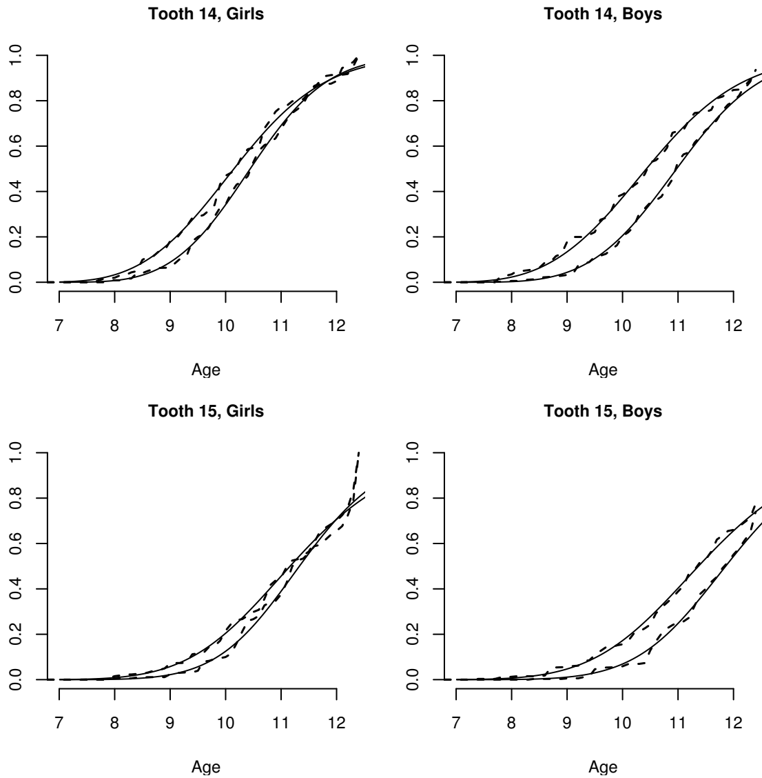
FIGURE 2. Predictive emergence curves: solid lines for curves based on the model gender * dm.f / scale(dm.f) (on each plot: left curve for dm.f = 1 , right curve for dm.f = 0 ), dashed line for a non-parametric estimate of Turnbull.
