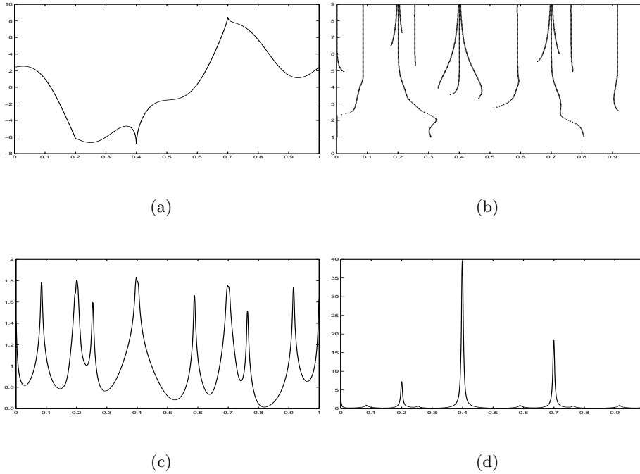
Figure 1: (a) Signal f_3 (see expression (2.3)). (b) Wavelet maxima of f_3 computed with a B-Spline of order 4 with r = 2 vanishing moments. (c) Non-weighted structural intensity of the wavelet maxima (d) Weighted structural intensity of the wavelet maxima.
