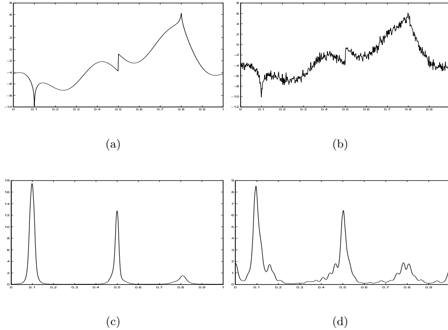
Figure 4: (a) Signal f_T (see expression (4.2)) (b) Noisy signal f_T with RSNR = 7, n = 512 . (c) EstWMS: structural intensity of the estimated wavelet maxima for r = 3 (d) DenSt: structural intensity of the wavelet maxima of \hat{f}_T (obtained by SureShrink thresholding) for r = 3
