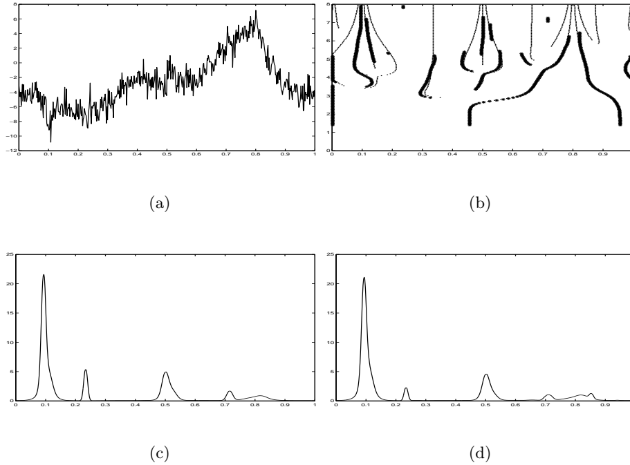
Figure 6: An example of bagging for removing spurious estimates: (a) Noisy signal f_T with RSNR = 3, n = 512 . (b) Estimated wavelet maxima (thick lines) and true wavelet maxima (thin lines) for r = 3 : note the presence of some spurious wavelet maxima at fine scales. (c) Weighted structural intensity of the estimated wavelet maxima. (d) Weighted structural intensity \hat{G}_m^{(Bag)}(x) of the estimated wavelet maxima after bagging
