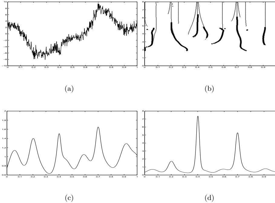
Figure 2: (a) Noisy signal f_3 with RSNR = 5 , n = 512 . (b) Estimated wavelet maxima (thick lines) and true wavelet maxima (thin lines) for r = 2 . (c) Non-weighted structural intensity of the estimated wavelet maxima (d) Weighted structural intensity of the estimated wavelet maxima
