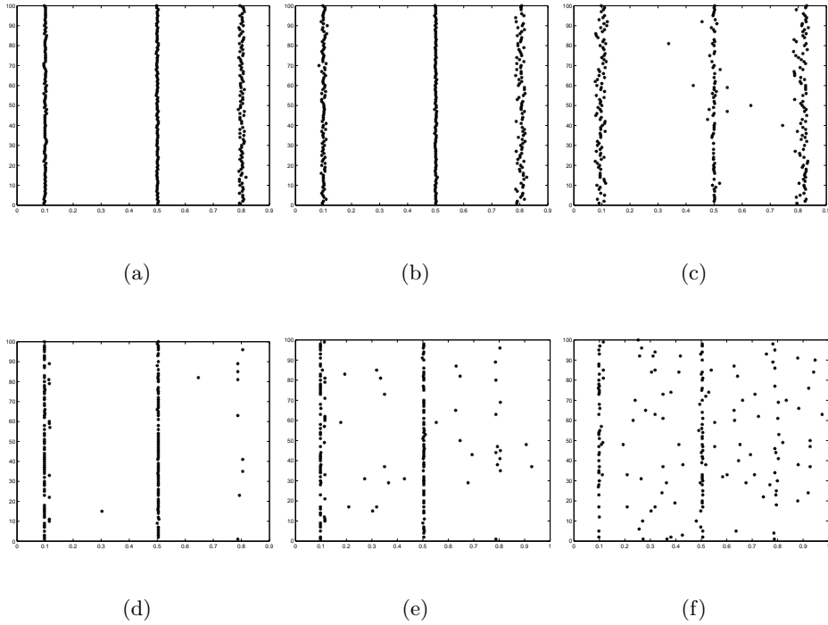
Figure 5: Locations of the significant modes of the structural intensity (with m_0 = 0.05 ) (a) EstWMSt RSNR = 7 , (b) EstWMSt RSNR = 5 , (c) EstWMSt RSNR = 3 , (d) DenSt RSNR = 7 , (e) DenSt RSNR = 5 , (f) DenSt RSNR = 3
