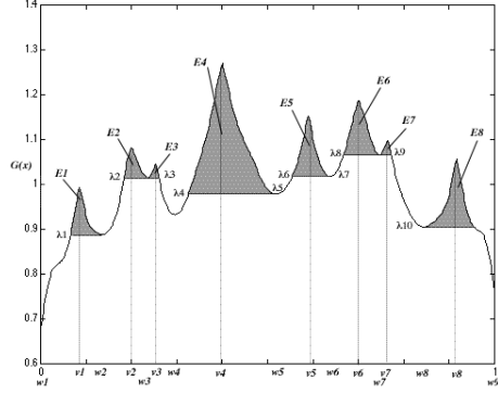
Figure 3: Structural intensity G(x) with a variety of modes. The shaded areas show the amount of mass E_j assigned to each mode. Each lower boundary \lambda_j is determined by the local minima of G(x) . The values v_1, v_2, \dots denote locations of successive maxima of G(x) and w_1, w_2, \dots denote locations of successive minima.
