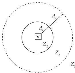
Fig. 4. Regions for distance fraud
