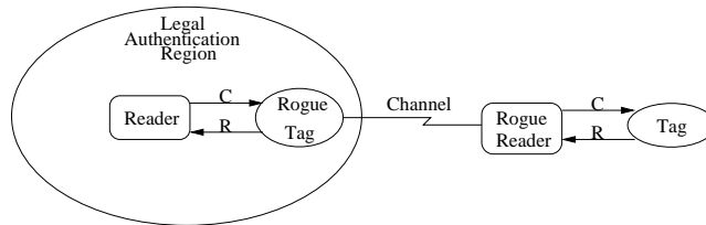
Fig. 1. A mafia fraud scenario
