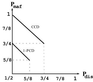
Fig. 5. Comparison of the trade-off curves for CCD and 1-PCD protocols
