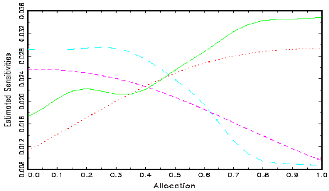
Figure 2 : Estimated sensitivity
