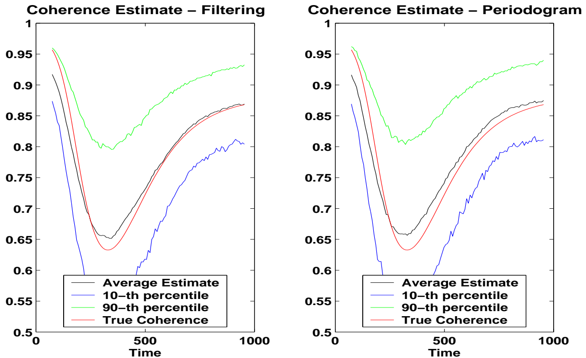
Figure 3: Band coherence for the non-stationary process. Plots of the 10-th percentile; 90-th percentile and average curves of the estimates from 1000 data sets obtained from the filtering method and the periodogram smoothing method.
