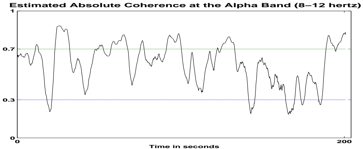
Figure 4: Estimate of the evolutionary absolute coherence between the EEGs at the T3 and P3 channels at the alpha band 8 – 12 hertz.
