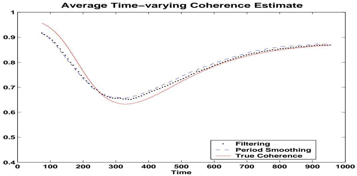
Figure 2: Band coherence for the non-stationary process. Plots of the true band coherence and average of the estimates from 1000 data sets obtained from the filtering method and the periodogram smoothing method.
