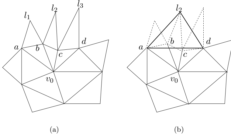
Figure 10: In (a), a R^2 -statistics superior to 90% has been detected. When computing f^{[2]} on the stencil belonging to \overline{\Omega}^{[2]} and having \{v_0, b, c\} as central triangle, the matrix to be inverted will be badly conditioned. In (b), we ignore for prediction the vertices b, c . Amongst the three flaps l_1, l_2, l_3 , we choose to keep in (b) the one with the smallest index ( l_2 in this case). This convention allows to always have a perfect reconstruction of a noise-free signal. In (b), the new neighborhood will produce a stable prediction. But the triangulation used is slightly different from the given Delaunay's triangulation (represented in dashed line).
