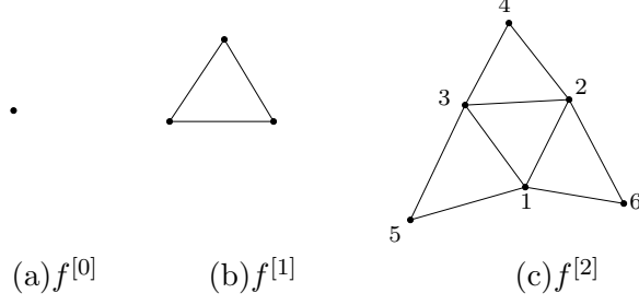
Figure 4: Stencils for divided differences.
