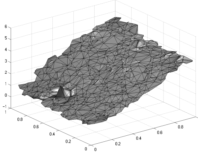
Figure 12: Estimation of the linear function (6.1) ( n = 700 , \text{SNR} = 2 ). The linear least squares predict operator is used, together with the minimum norm update followed by semi-orthogonalization. The efficiency \text{Eff} obtained for this estimate is equal to 3.273.
